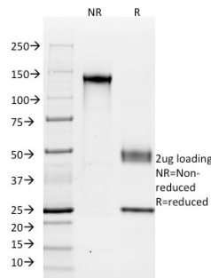
SDS-PAGE Analysis of Purified KSP-Cadherin Mouse Monoclonal Antibody (SPM594). Confirmation of Purity and Integrity of Antibody.
