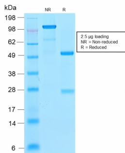
SDS-PAGE Analysis of Purified p21 Rabbit Recombinant Monoclonal Antibody (CIP1/2275R).
