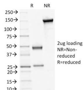
SDS-PAGE Analysis of Purified Desmoglein-3 Monoclonal Antibody (5H10). Confirmation of Integrity and Purity of Antibody.
