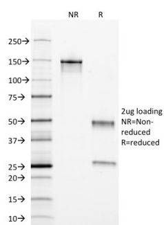
SDS-PAGE Analysis of Purified Ferritin, Light Chain Mouse Monoclonal Antibody (FTL/1389). Confirmation of Integrity and Purity of Antibody
