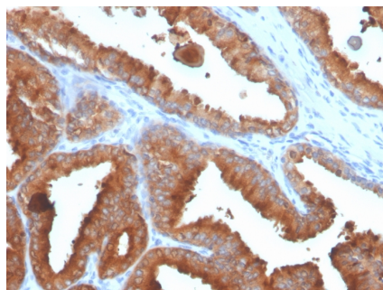
Formalin-fixed, paraffin-embedded human prostate carcinoma stained with PSA Recombinant Mouse Monoclonal Antibody (rKLK3/4753).
