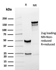
SDS-PAGE Analysis of Purified PSA Recombinant Mouse Monoclonal Antibody (rKLK3/4753). Confirmation of Integrity and Purity of Antibody.
