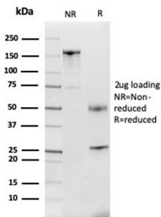
SDS-PAGE Analysis Lactoferrin Mouse Monoclonal Antibody (LTF/4079). Confirmation of Purity and Integrity of Antibody.
