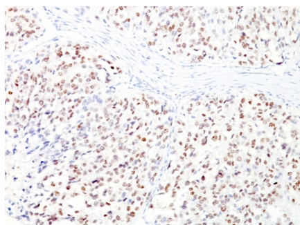
Formalin-fixed, paraffin-embedded human Melanoma stained with MITF Monoclonal Antibody (D5 + MITF/915).
