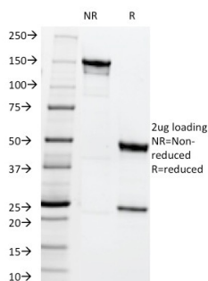
SDS-PAGE Analysis of Purified MRP1 Mouse Monoclonal Antibody (MRP1/1344). Confirmation of Integrity and Purity of Antibody.
