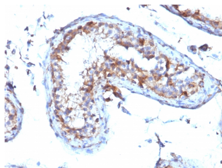
Formalin-fixed, paraffin-embedded human Testicular Carcinoma stained with Moesin Mouse Monoclonal Antibody (MSN/492).
