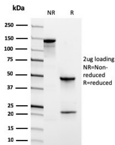
SDS-PAGE Analysis Purified CD31 Mouse Monoclonal Antibody (PECAM1/3526). Confirmation of Integrity and Purity of Antibody.
