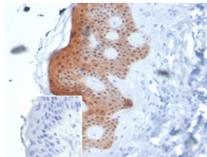
Formalin-fixed, paraffin-embedded human skin stained with SERPINB5 / Maspin Mouse Monoclonal Antibody (SERPINB5/4975). Inset: PBS instead of primary antibody; secondary only negative control.
