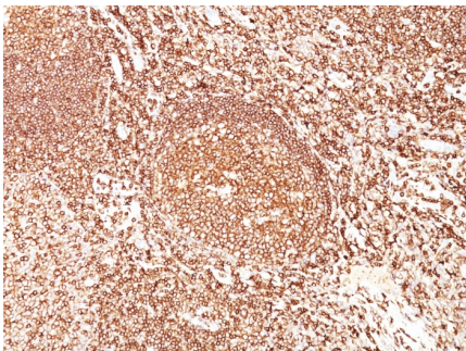
Formalin-fixed, paraffin-embedded human tonsil stained with CD45 / LCA Mouse Monoclonal Antibody (F10-89-4).
