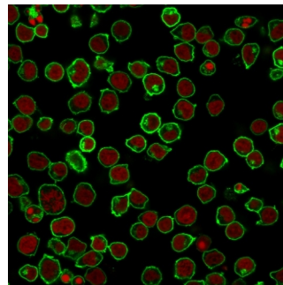
Immunofluorescence Analysis of PFA-fixed Jurkat cells labeling CD45. CD45 / LCA Mouse Monoclonal Antibody (F10-89-4) followed by goat anti-mouse IgG-CF488 (green). Nuclear counterstain is RedDot.
