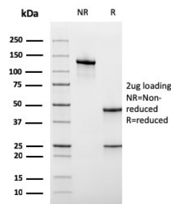
SDS-PAGE Analysis of Purified CD45RA Monoclonal Antibody (rPTPRC/1131). Confirmation of Purity and Integrity of Antibody.
