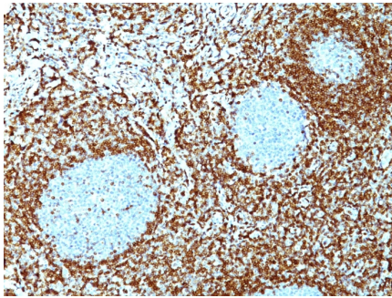
Formalin-fixed, paraffin-embedded non-Hodgkin's lymphoma stained with Bcl-2 Mouse Monoclonal Antibody (100/D5 + 124). Note nuclear membrane & cytoplasmic staining.
