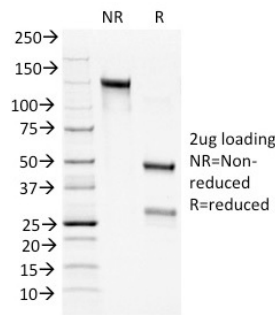
SDS-PAGE Analysis of Purified Bcl-2 Mouse Monoclonal Antibody (100/D5 + 124). Confirmation of Integrity and Purity of Antibody.
