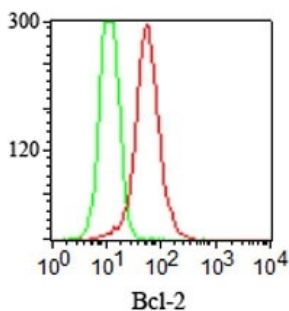
Intracellular staining of Bcl-2 in Jurkat cells using Bcl-2 Mouse Monoclonal Antibody (100/D5 + 124). (red) and isotype control (green).
