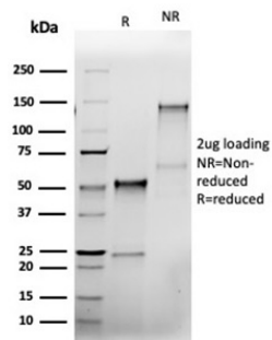
SDS-PAGE Analysis of Purified Bcl-x Recombinant Mouse Monoclonal Antibody (rBCL2L1/4508). Confirmation of Purity and Integrity of Antibody.
