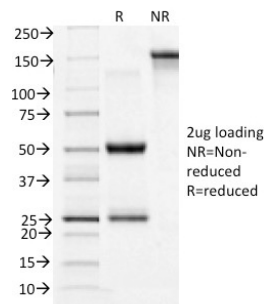
SDS-PAGE Analysis of Purified CD71 Mouse Monoclonal Antibody (TFRC/1396). Confirmation of Integrity and Purity of Antibody.
