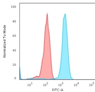
Flow Cytometric Analysis of human Jurkat cells using CD71 Mouse Monoclonal Antibody (TFRC/1396) followed by Goat anti-Mouse IgG-CF488 (Blue); Isotype Control (Red).
