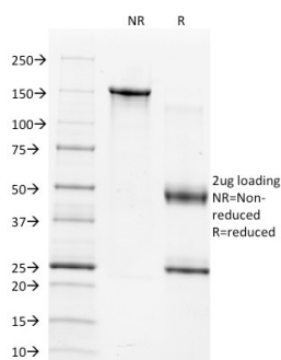
SDS-PAGE Analysis of Purified TIMP1 Mouse Monoclonal Antibody (2A5). Confirmation of Integrity and Purity of Antibody.
