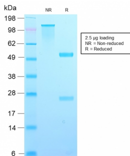
SDS-PAGE Analysis of Purified TIMP2 Rabbit Recombinant Monoclonal Antibody (TIMP2/2488R). Confirmation of Integrity and Purity of Antibody.
