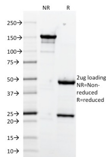
SDS-PAGE Analysis of Purified CD106 Monoclonal Antibody (1.4C3). Confirmation of Purity and Integrity of Antibody.
