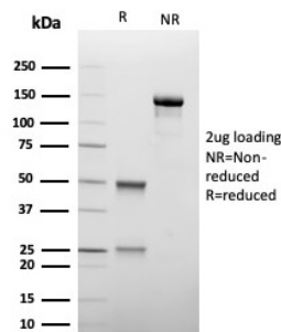
SDS-PAGE Analysis of Purified TIM3 Mouse Monoclonal Antibody (TIM3/4027). Confirmation of Integrity and Purity of Antibody.
