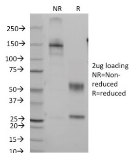
SDS-PAGE Analysis of Purified CD7 Mouse Monoclonal Antibody (Clone B-F12). Confirmation of Integrity and Purity of Antibody.
