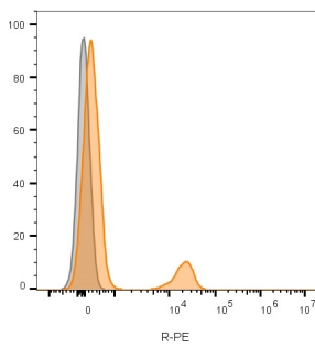
Flow cytometric analysis of lymphocyte-gated PBMCs. CD19 Mouse Monoclonal Antibody (CVID3/155) labeled with CF568 (orange); unstained cells (gray).
