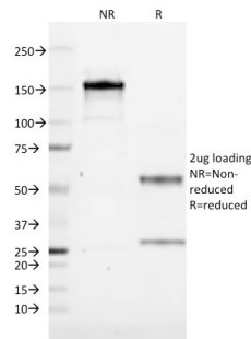
SDS-PAGE Analysis of Purified CD19 Mouse Monoclonal Antibody (CVID3/155). Confirmation of Integrity and Purity of Antibody.
