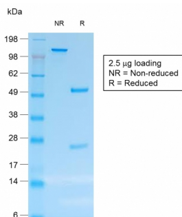
SDS-PAGE Analysis of Purified CD30 Mouse Recombinant Monoclonal Antibody (rCD30/412). Confirmation of Purity and Integrity of Antibody.
