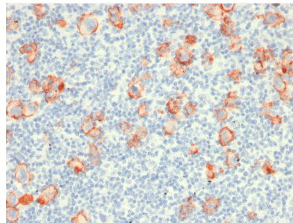
Formalin-fixed, paraffin-embedded human Hodgkin's lymphoma stained with CD30 Mouse Recombinant Monoclonal Antibody (rCD30/412).
