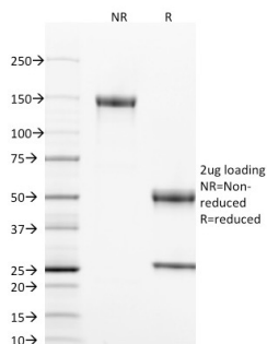
SDS-PAGE Analysis of Purified CD40 Mouse Monoclonal Antibody (T8P2G4*A6). Confirmation of Integrity and Purity of Antibody.
