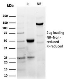
SDS-PAGE Analysis of Purified CD40 Recombinant Rabbit Monoclonal Antibody (C40/4826R). Confirmation of Integrity and Purity of Antibody.
