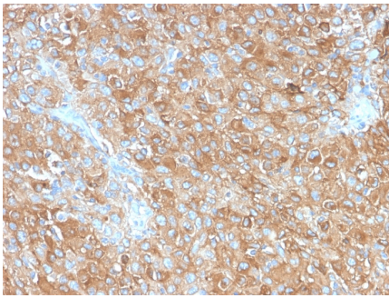
Formalin-fixed, paraffin-embedded human Prostate Carcinoma stained with CD63 Rabbit Recombinant Monoclonal Antibody (LAMP3/2990R).
