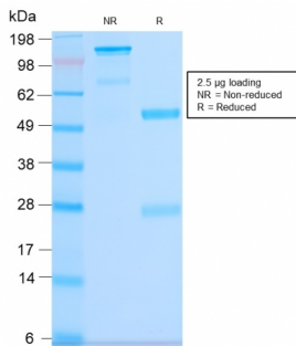
SDS-PAGE Analysis of Purified CD63 Rabbit Recombinant Monoclonal Antibody (LAMP3/2990R). Confirmation of Purity and Integrity of Antibody.
