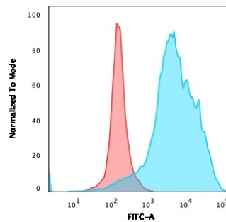
Flow Cytometric Analysis of PFA-fixed U87MG cells. CD63 Rabbit Recombinant Monoclonal Antibody (LAMP3/2990R) followed by goat anti-rabbit IgG-CF488 (Blue); Isotype Control (Red).
