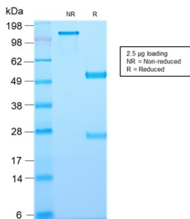
SDS-PAGE Analysis of Purified CD81 Rabbit Recombinant Monoclonal Antibody (C81/2885R). Confirmation of Purity and Integrity of Antibody.
