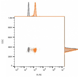
Flow cytometry analysis of bead-bound exosomes derived from MCF-7 cells. Unstained exosomes (gray) or exosomes stained with CF568-labeled CD81 monoclonal antibody (2885R) (orange).
