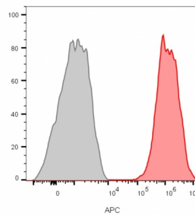
Flow cytometry analysis of MCF-7 cells unstained (gray) or stained with CD81 Rabbit Recombinant Monoclonal Antibody (C81/2885R) and goat anti-mouse CF647 (red).
