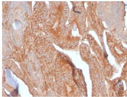
Formalin-fixed, paraffin-embedded human Prostate Carcinoma stained with CD81 Rabbit Recombinant Monoclonal Antibody (C81/2885R).
