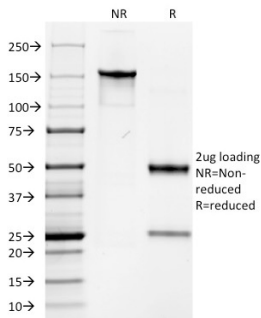
SDS-PAGE Analysis of Purified Cytokeratin, HMW Mouse Monoclonal Antibody (AE-3). Confirmation of Purity and Integrity of Antibody.
