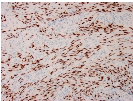
Formalin-fixed, paraffin-embedded human Kaposi's sarcoma stained with HHV8 Recombinant Rabbit Monoclonal Antibody (HHV8/3633R).
