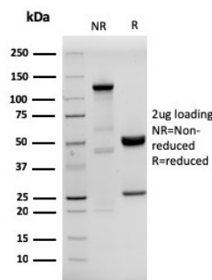
SDS-PAGE Analysis of Purified HHV8 Recombinant Rabbit Monoclonal Antibody (HHV8/3633R). Confirmation of Purity and Integrity of Antibody.
