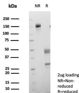
SDS-PAGE Analysis of Purified GLUT-1 Mouse Monoclonal Antibody (GLUT1/7308). Confirmation of Purity and Integrity of Antibody.
