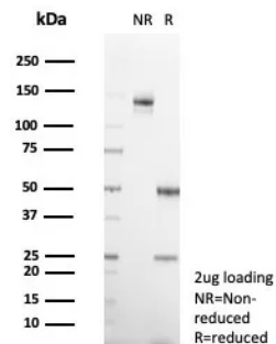
SDS-PAGE Analysis of Purified Interleukin-1 Beta (IL-1B) Mouse Monoclonal Antibody (IL1B/4650). Confirmation of Purity and Integrity of Antibody.
