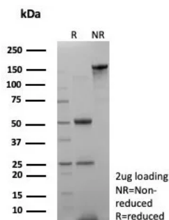
SDS-PAGE Analysis of Purified SHBG Mouse Monoclonal Antibody (SHBG/8175). Confirmation of Integrity and Purity of Antibody.
