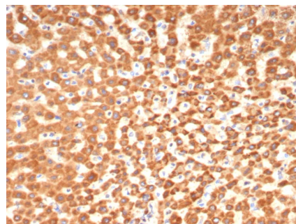
Formalin-fixed, paraffin-embedded human hepatocellular carcinoma stained with SHBG Mouse Monoclonal Antibody (SHBG/8175). HIER: Tris/EDTA, pH9.0, 45min. 2°C: HRP-polymer, 30min. DAB, 5min.
