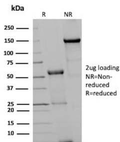
SDS-PAGE Analysis of Purified CD276 Mouse Monoclonal Antibody (B7H3/4479). Confirmation of Purity and Integrity of Antibody.
