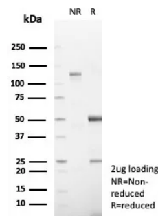
SDS-PAGE Analysis of Purified DSG3 Recombinant Rabbit Monoclonal Antibody (DSG3/8252R). Confirmation of Integrity and Purity of Antibody.
