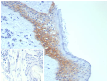
Formalin-fixed, paraffin-embedded human skin stained with Desmoglein-3 Recombinant Rabbit Monoclonal Antibody (DSG3/8252R). Inset: PBS instead of primary antibody; secondary only negative control.
