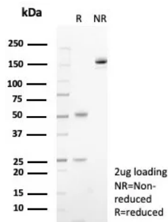
SDS-PAGE Analysis of Purified CD23 Recombinant Rabbit Monoclonal Antibody (FCER2/8236R). Confirmation of Purity and Integrity of Antibody.
