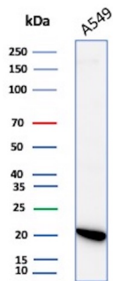
Western blot analysis of A549 lysate using IL-18 Mouse Monoclonal Antibody (IL18/4626).
