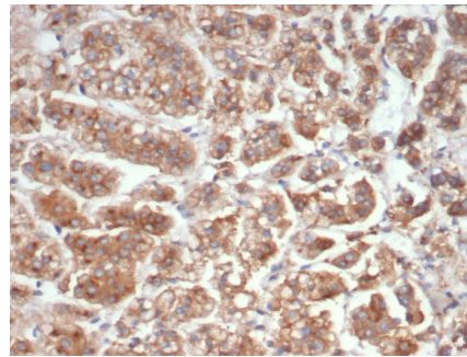
Formalin-fixed, paraffin-embedded human adrenal gland stained with IL-18 Mouse Monoclonal Antibody (IL18/4626). HIER: Tris/EDTA, pH9.0, 45min. 2°C: HRP-polymer, 30min. DAB, 5min.
