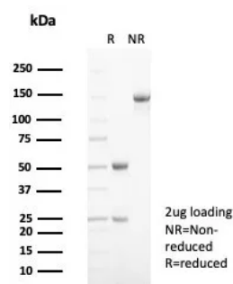
SDS-PAGE Analysis of Purified CD99 Mouse Monoclonal Antibody (MIC2/7863). Confirmation of Purity and Integrity of Antibody.
