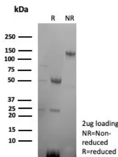
SDS-PAGE Analysis of Purified CD2 Recombinant Rabbit Monoclonal Antibody (LFA2/8845R). Confirmation of Purity and Integrity of Antibody.
