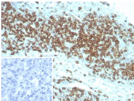
Formalin-fixed, paraffin-embedded human lymph node stained with CD2 Recombinant Rabbit Monoclonal Antibody (LFA2/8845R). HIER: Tris/EDTA, pH9.0, 45min. 2°C: HRP-polymer, 30min. DAB, 5min.
