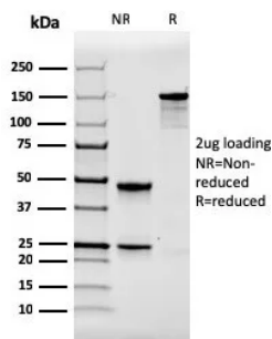
SDS-PAGE Analysis of Purified Tryptase Recombinant Mouse Monoclonal Antibody (rTPSAB1/1963). Confirmation of Purity and Integrity of Antibody.
